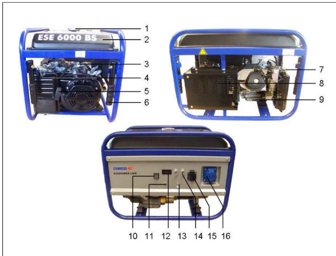
Fig. 3.1: Components of the generator
