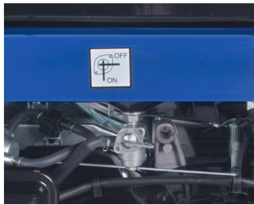
Fig. 4.1: Open/close fuel valve
