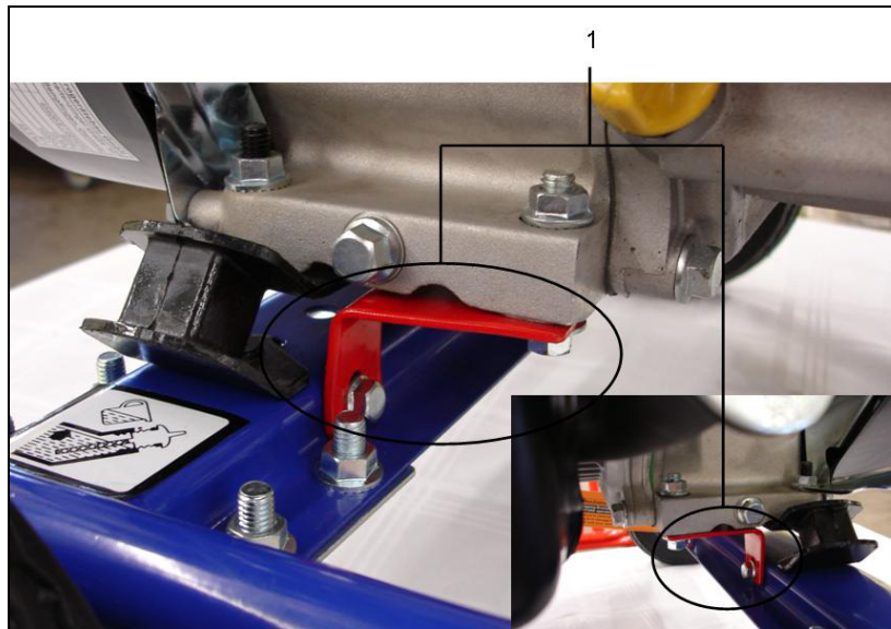
Figure 2: Transport safety device
